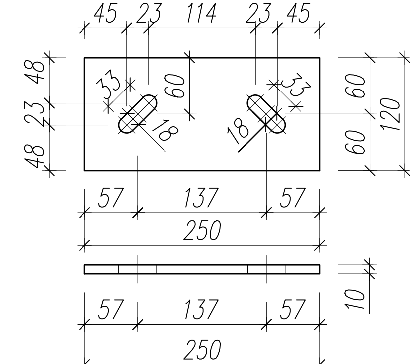
ELEMENT "A2"
