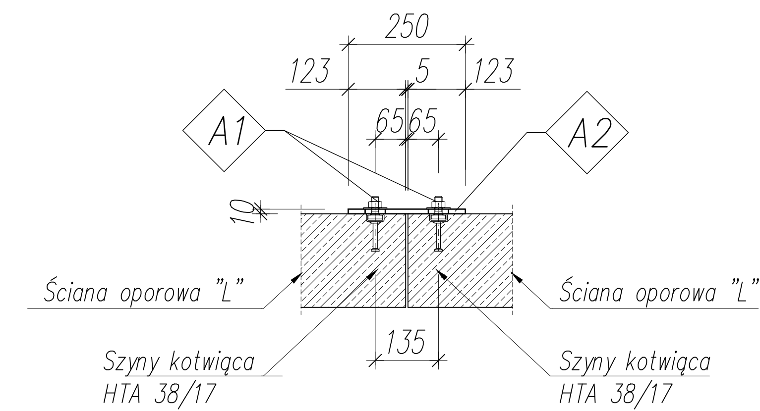
DETAL "A"
